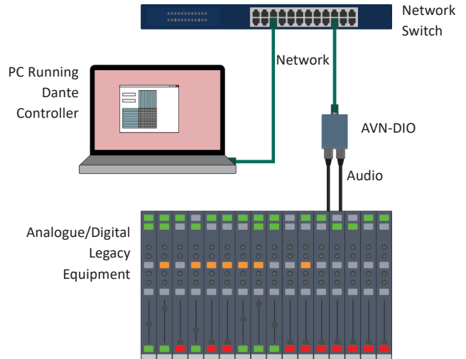
Fig 10: Typical AVN-DIO setup
