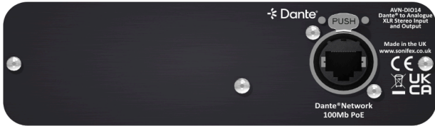
Fig 3: AVN-DIO14 Rear Panel
