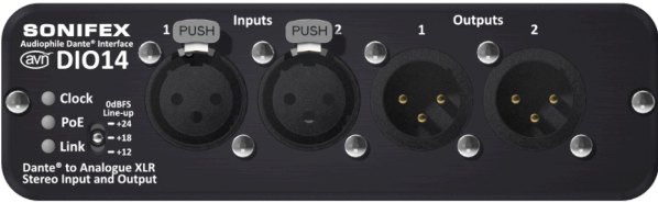
Fig 2: AVN-DIO14 Front Panel
